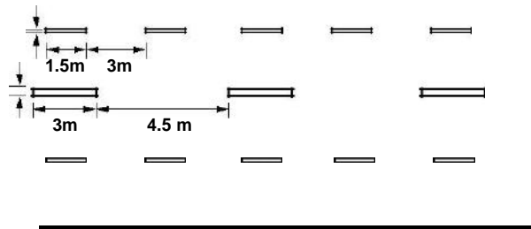
Figure 37:2: Centre line and lane marking for a four lane road
